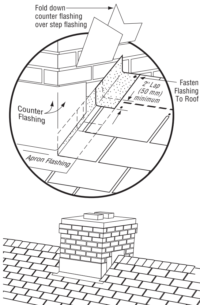
Figure 12-10: Flashing around a chimney.
