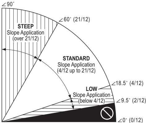
Figure 12-1: Slope definitions.
