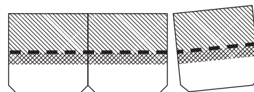
Figure 12-11: Shadow Ridge shingles detach easily from three-piece units to make 72 individual cap pieces.
