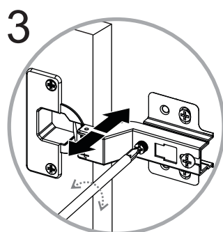
side adjustment
