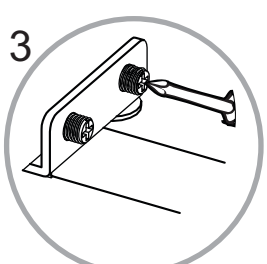
Insert pivot and lower glass door hinge
