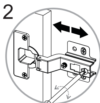
Depth adjustment
