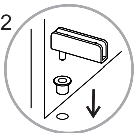
Insert pivot and upper glass door hinge
