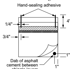
Figure 18-14: Hand seal caps
