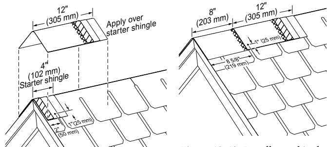
Figure 18-12: Apply a full cap shingle over the starter shingle.
