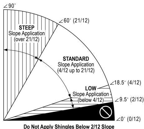
Figure 18-1: Slope definitions.
