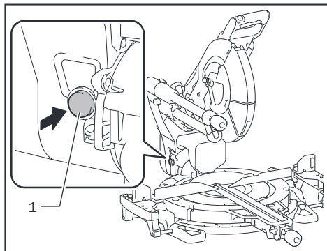
► 1. Releasing button
