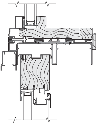
HORIZONTAL JOINING MULLION TRANSOM / LIFESTYLE SLIDING DOOR (FIXED)
