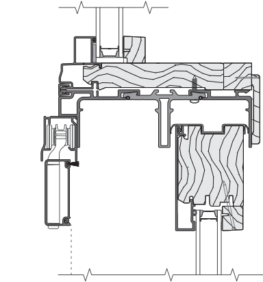
HORIZONTAL JOINING MULLION TRANSOM / SLIDING DOOR (VENT)
