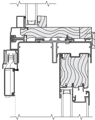
HORIZONTAL JOINING MULLION TRANSOM / LIFESTYLE SLIDING DOOR (VENT)
