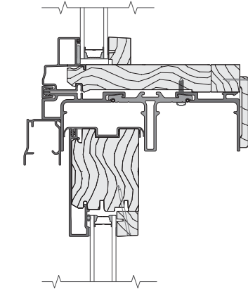
HORIZONTAL JOINING MULLION TRANSOM / SLIDING DOOR (FIXED)
