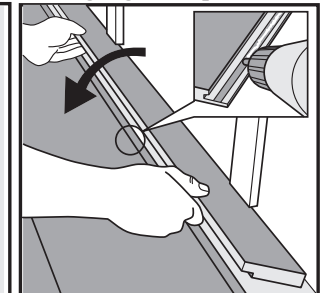
Fig.15 Put glue along the modified locking profile, press the panels together and weight until glue is dry. Use a pull bar to remove any gaps.
