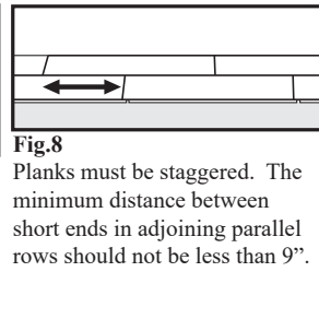
Fig.8 Planks must be staggered. The minimum distance between short ends in adjoining parallel rows should not be less than 9".
