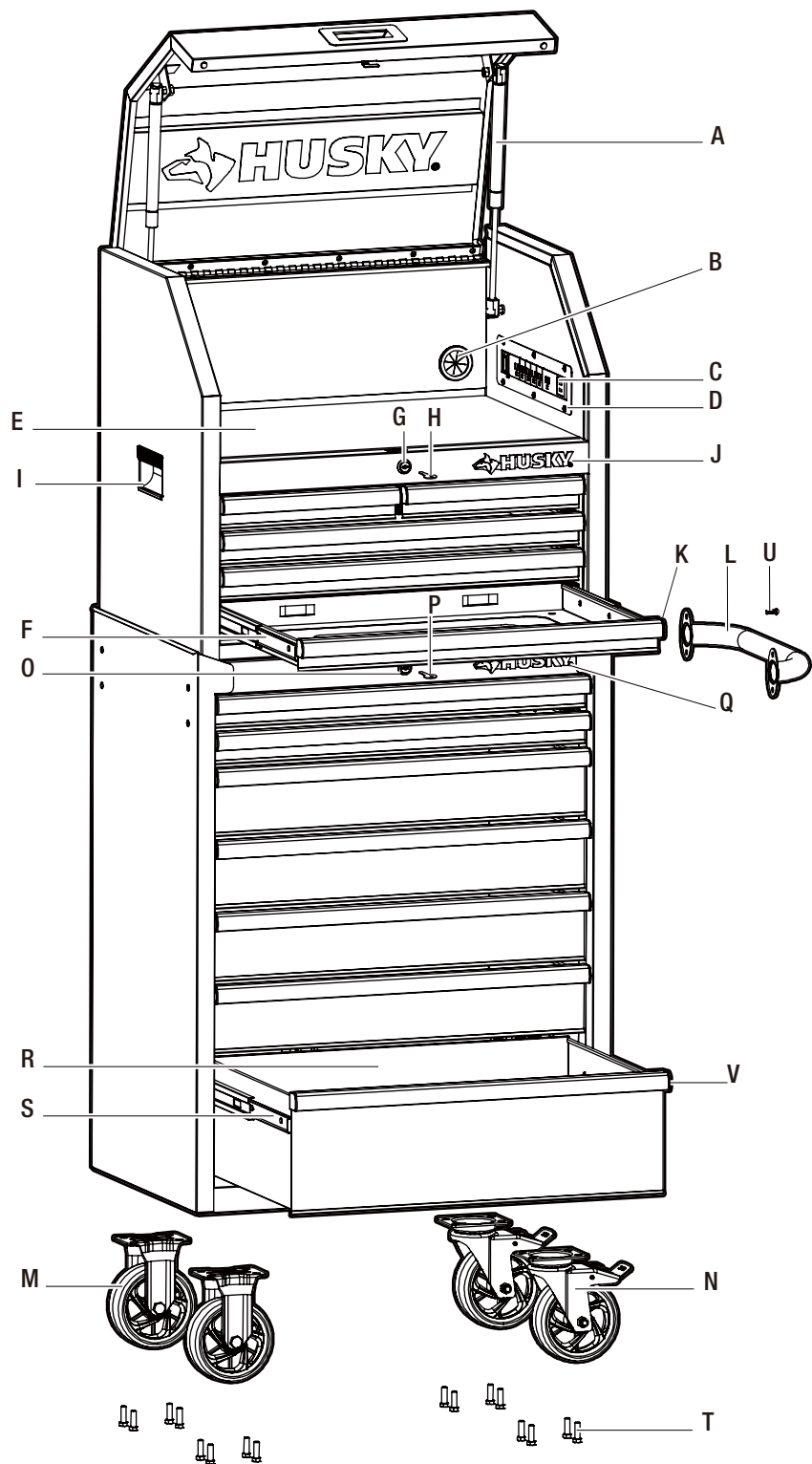
Cabinet
