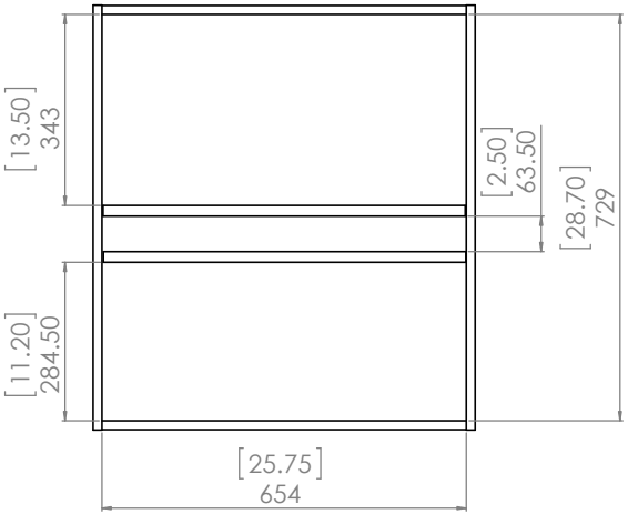
Front View (front doors removed)
