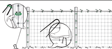
INSTALLATION WITH WOODEN POST
