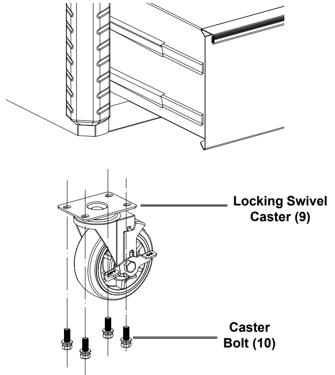
Figure B: Caster Attachment
