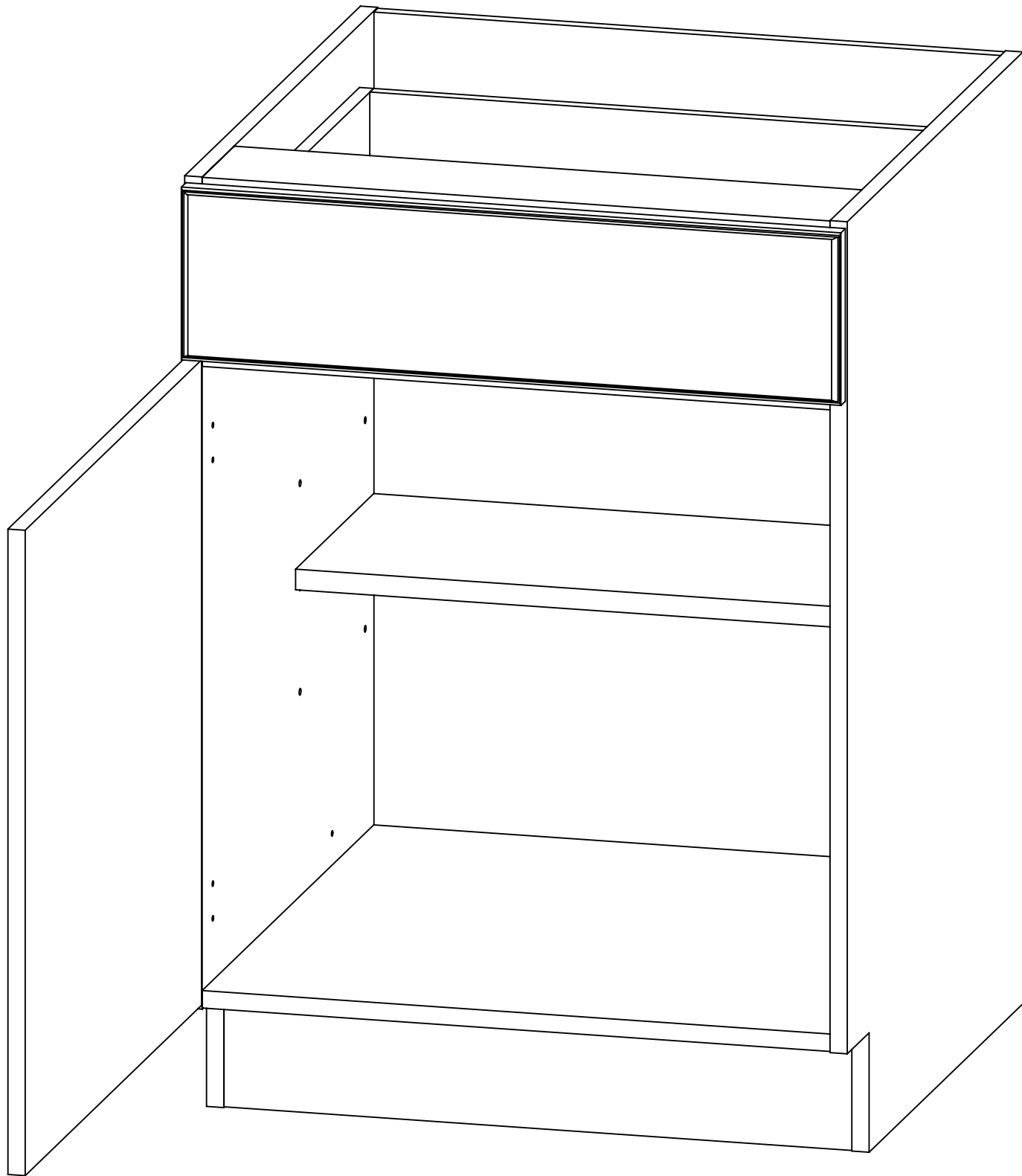
Isometric View
