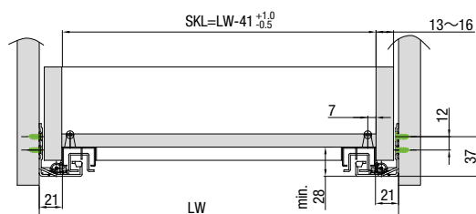
Drawer width
