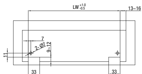
Drawer back drilling and notching
