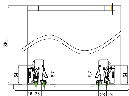
Locking device mounting
