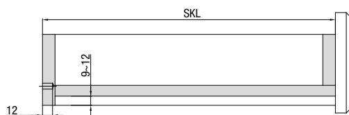
Drawer length
