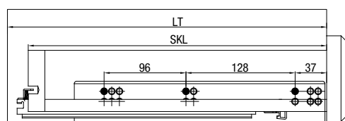
Drawer vs. cabinet length
