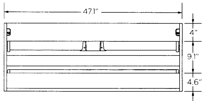
Cabinet Back
