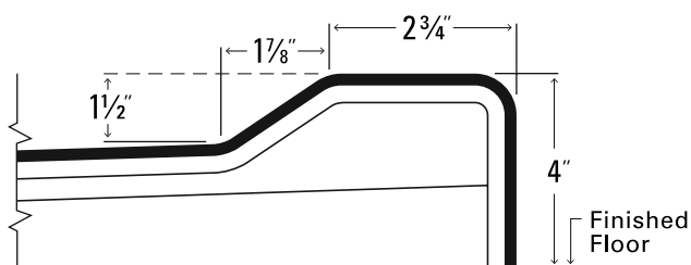
4" LOW THRESHOLD
